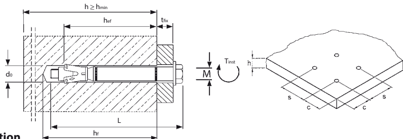
Dimensions countersunk head SZ-SK [mm]
